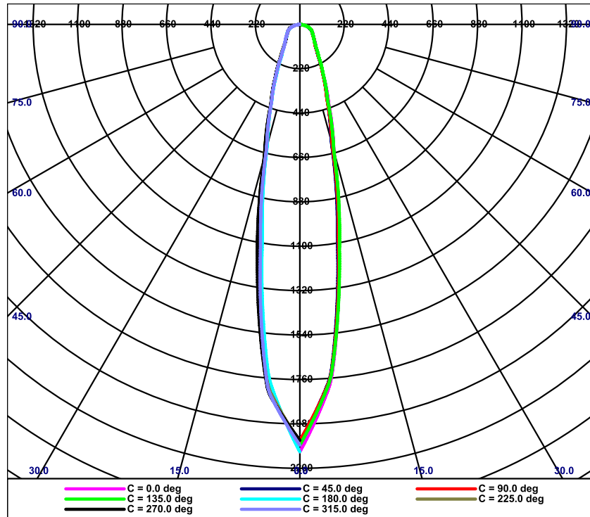
Polar Luminous Intensity Distribution
