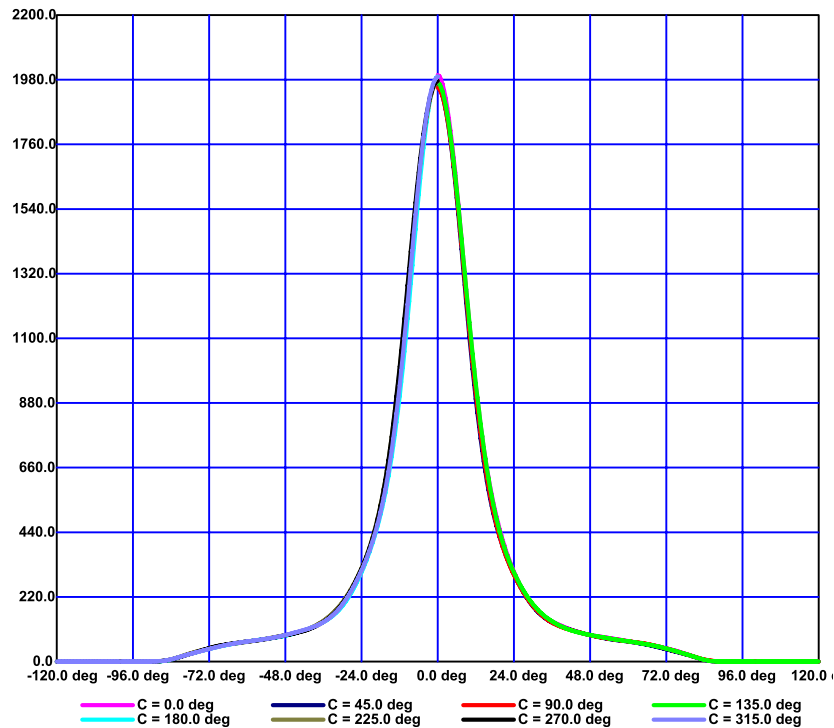
Cartesian Luminous Intensity Distribution
